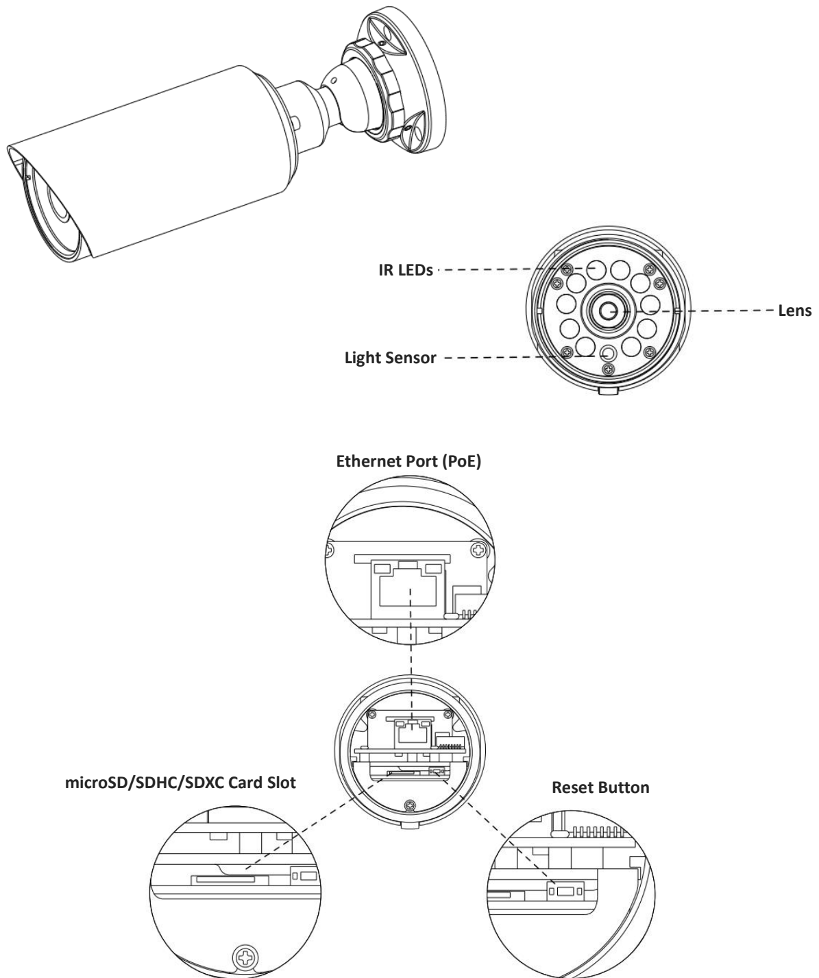
Figure 1-3-6 Mini Bullet Network Camera
